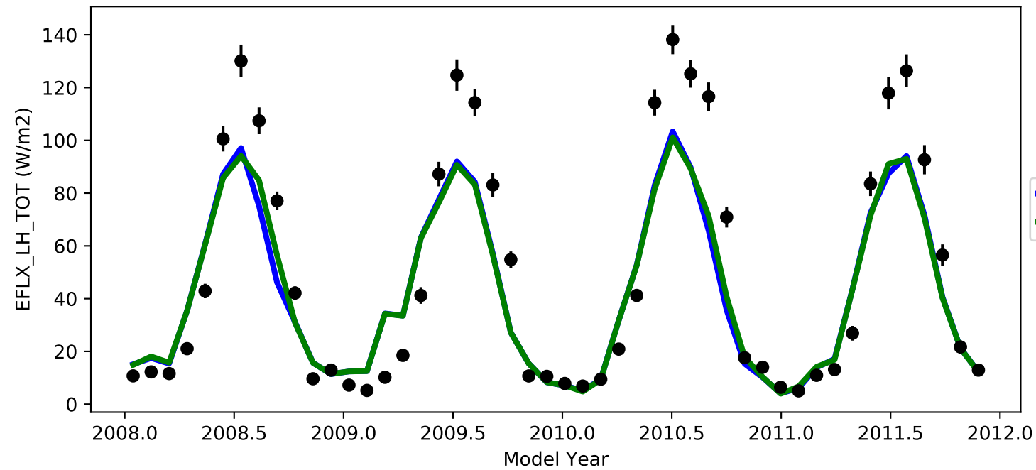
total latent heat flux [+ to atm]
